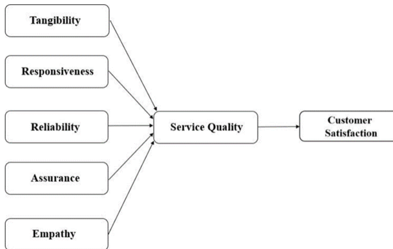
Figure 1. SERVQUAL model.
